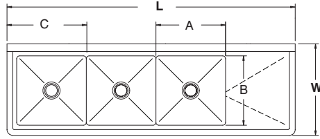
3 COMP - 1 DRBD
