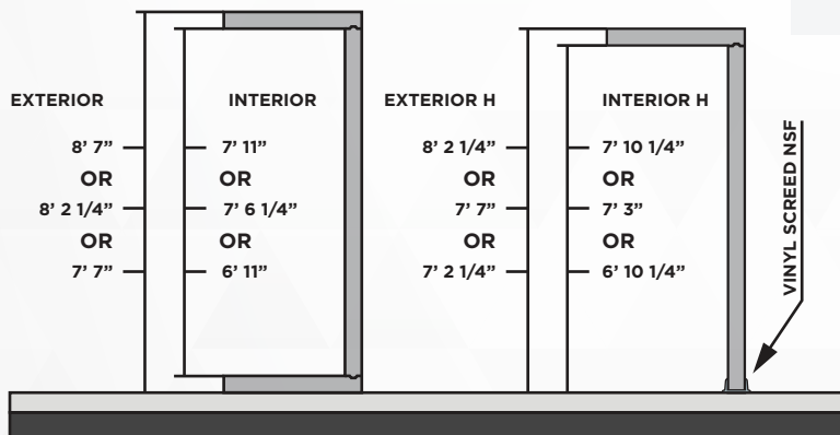
SIDE VIEW WITH FLOOR (RECOMMENDED FOR FREEZERS)
