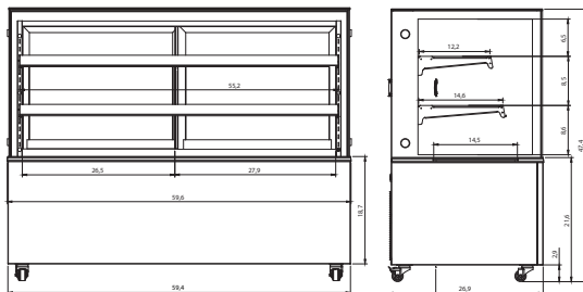
KBF-60 KBF-60D
