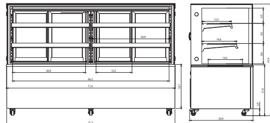
KBF-72 KBF-72D
